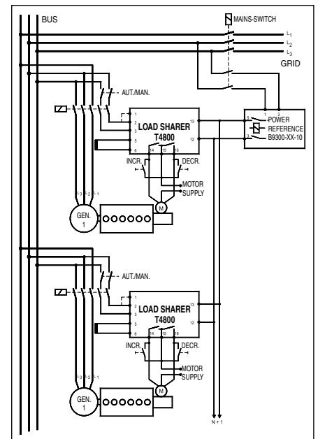
Fig. 2. Application Diagram. B9300 with T4800.
