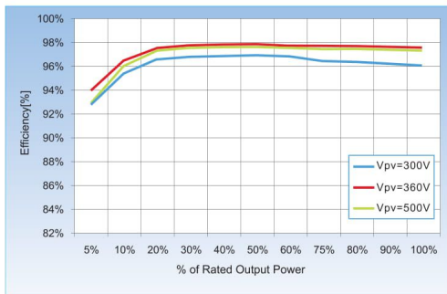
Efficiency Curve
